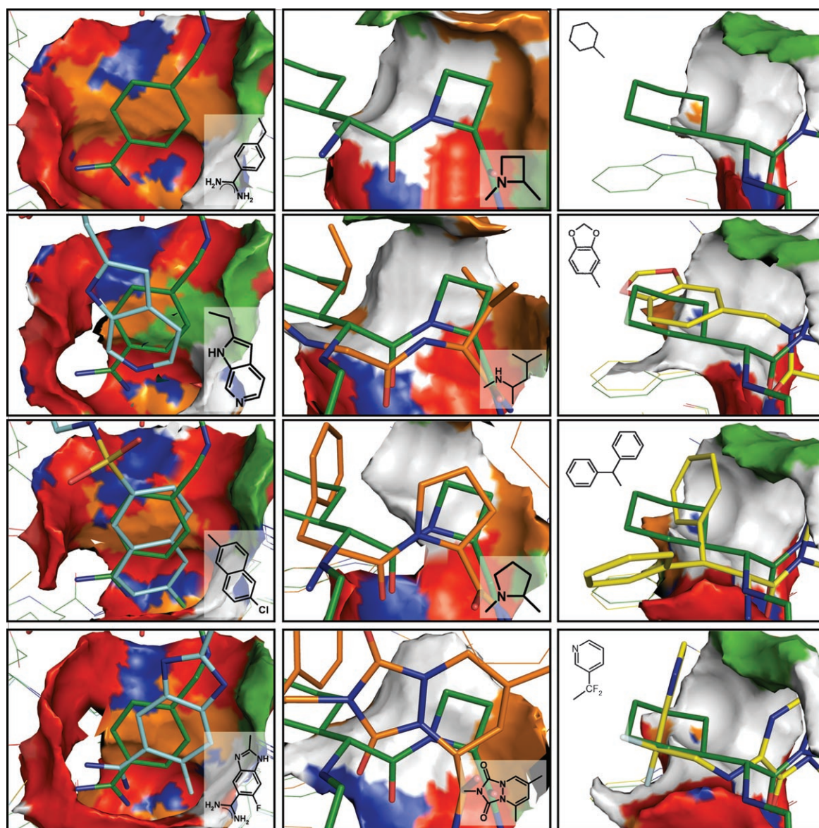
Figure 1. Fragments found by subcavity matching. For comparison, the crystallographically determined binding mode of melagatran (green, PDB code 1k22) in thrombin [9] is shown in the upper row for the S1 (left), S2 (center), and S3 (right) pocket together with three examples retrieved from occupants in other proteins (second to fourth rows). These protein surfaces display similar physicochemical properties (blue: H-bond donor, red: H-bond acceptor, green: donor or acceptor, white and orange: areas for interaction with aliphatic and aromatic groups, respectively). In the first row, the physicochemical properties for the melagatran complex are shown. In the following rows, the physicochemical properties of the subcavities in the other proteins matched by the algorithm are displayed. The adopted binding geometry (cyan, orange, yellow) and chemical formulas of the fragments occupying the corresponding subpockets are given.
