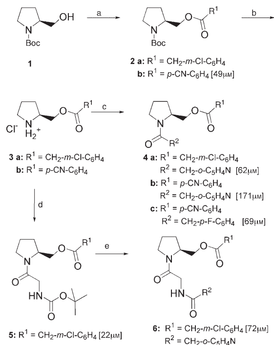
Scheme 3. Synthesis of compounds 2–6. K_i values for 2b, 4a, 4b, 4c, 5, and 6 for thrombin inhibition are given in square brackets. Reagents and reaction conditions are given in the Supporting Information.
