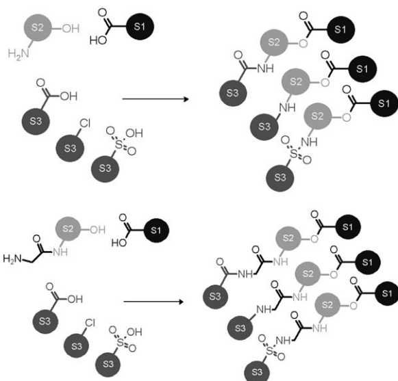
Scheme 2. Synthetic route for the assembly of the virtual combinatorial library by means of FlexX C .
