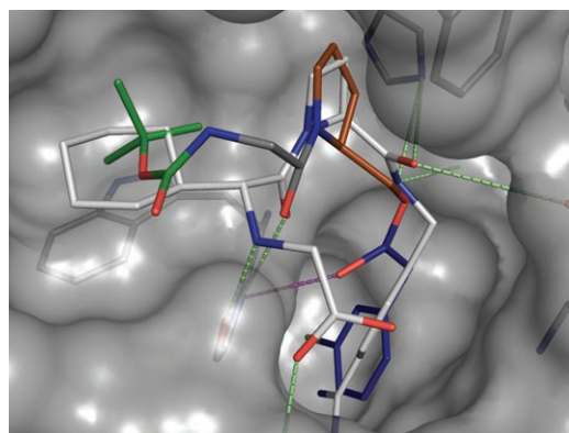
Figure 2. Superposition of the crystal structure of 5 (P1: 3-chlorobenzyl portion in blue; P2: prolinol moiety in brown, glycine spacer in dark gray; P3: tert -butyl moiety in green) with melagatran (extracted from PDB code 1k22). Melagatran (gray) forms by its P1–P2 amide-bond H-bonds (light green) to Ser195 and Glu192. Furthermore, it involves Gly216 in a double hydrogen bond. In contrast, in compound 5, the formation of an optimal H-bond network between protein and bound ligand is perturbed by interaction between the ester carbonyl oxygen atom and the Gly216 NH group (magenta).
