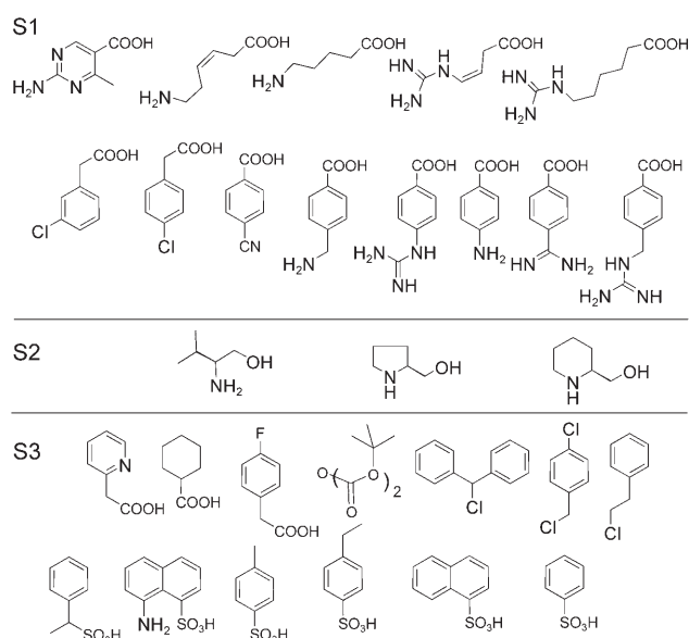
Scheme 1. Chemical formulas of the building blocks for the three subpockets.
